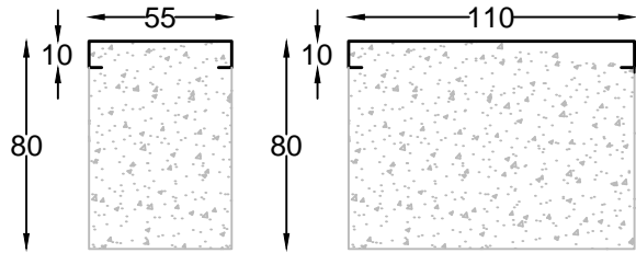
B1 SQR 8-55/10
