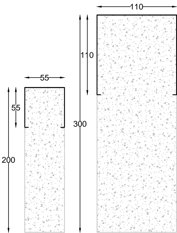
B2 SQR 20-55/55
